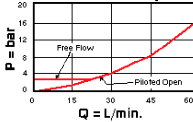
Free Flow and Piloted Open Pressure Drop
